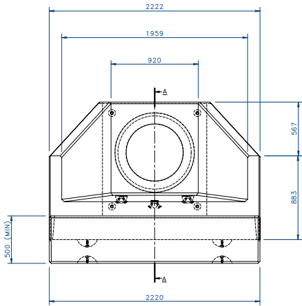
Spillway Headwall S60
