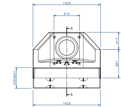
Spillway Headwall S40
