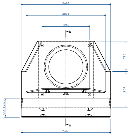
Spillway Headwall S90
