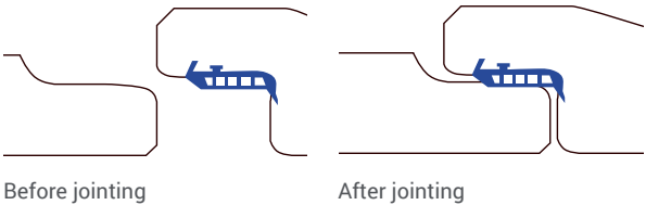
Integral seal - lubricated
